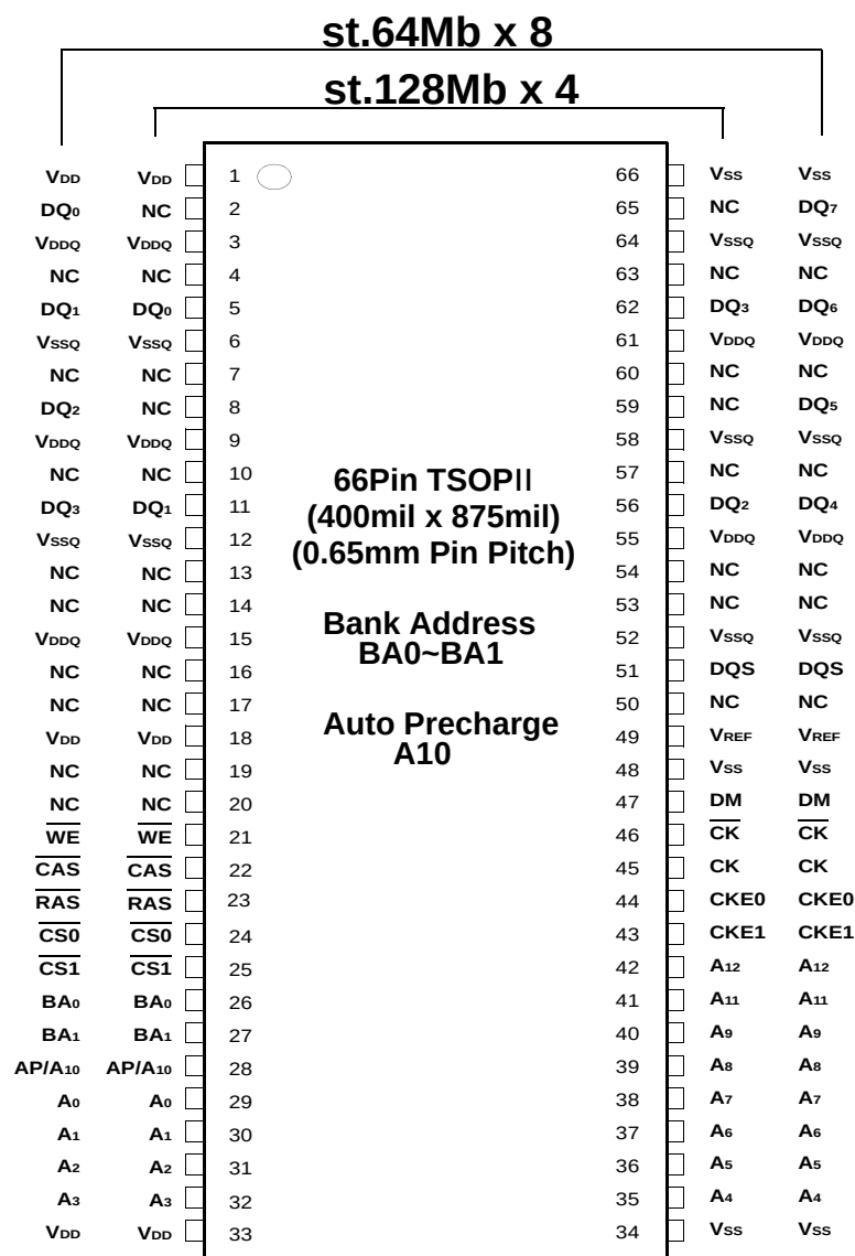
stacked 512Mb TSOP-II Package Pinout
