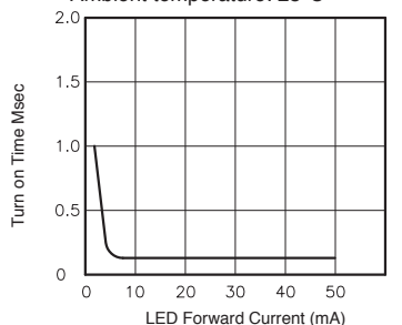
Fig.10 LED forward current vs. turn on time Across terminals 4 and 6 pin; Load voltage: 400V (DC); Continuous load current: 130mA (DC); Ambient temperature: 25°C
