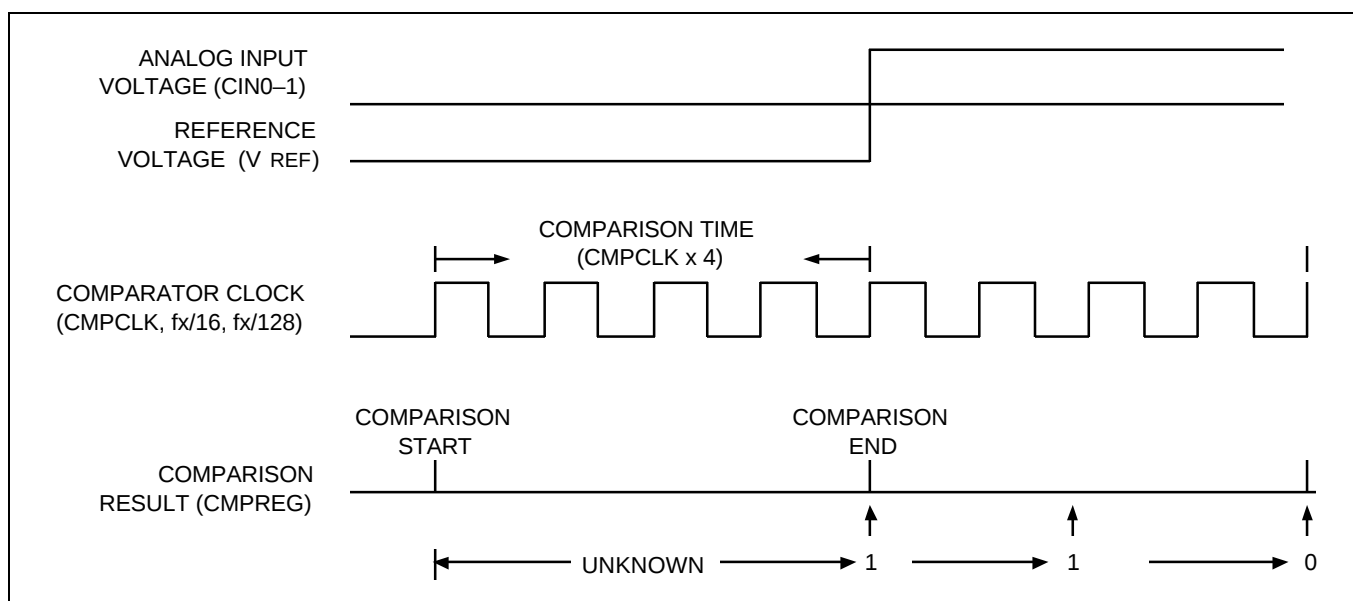
Figure 44. Conversion Characteristics
