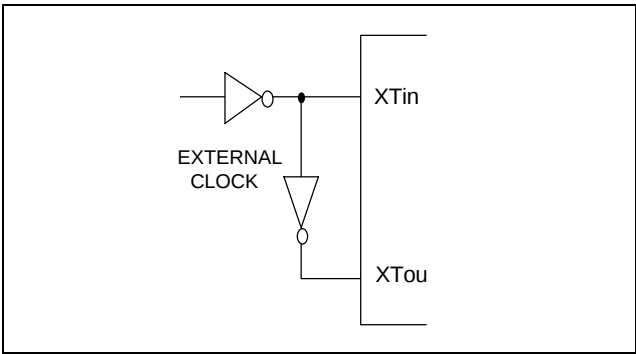
Figure 18. External Oscillator (fx)
