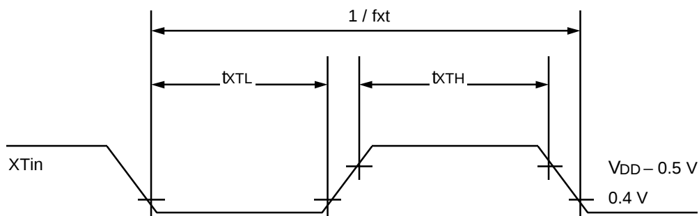
Figure 53. Clock Timing Measurement at XT_{in}
