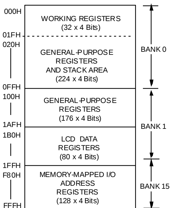
Figure 14. Data Memory (RAM) Map
