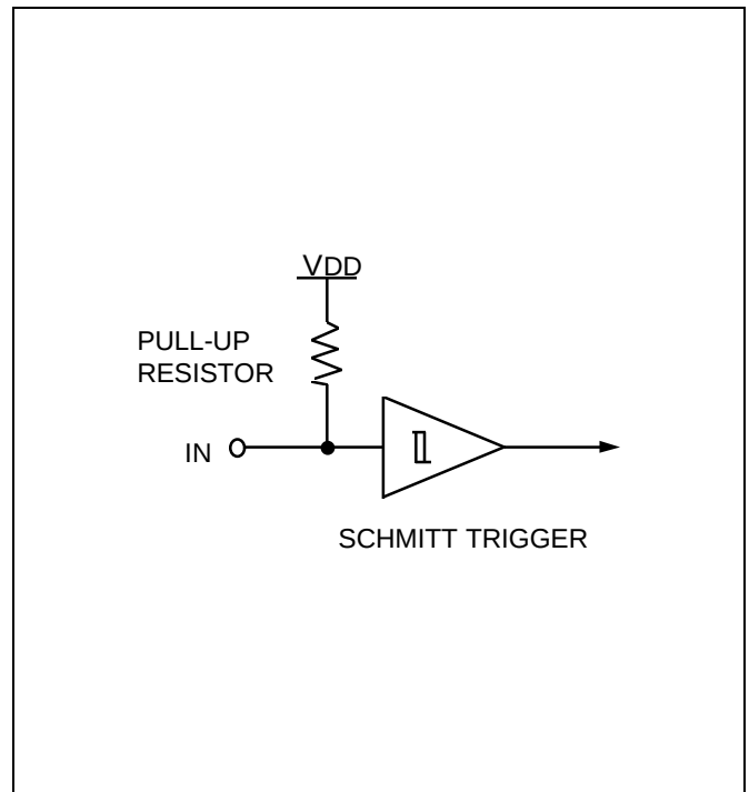
Figure 4. Pin Circuit Type 2
