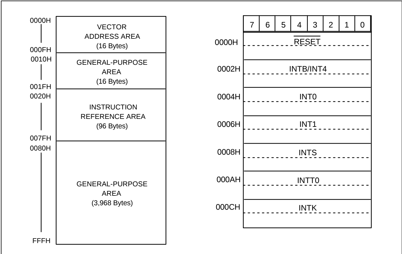
Figure 13. ROM Address Structure
