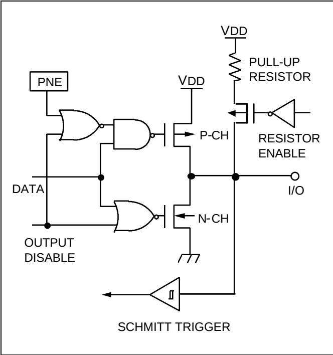
Figure 8. Pin Circuit Type 6
