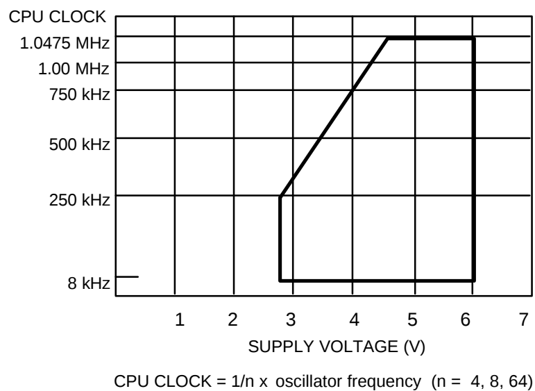
Figure 48. Standard Operating Voltage Range
