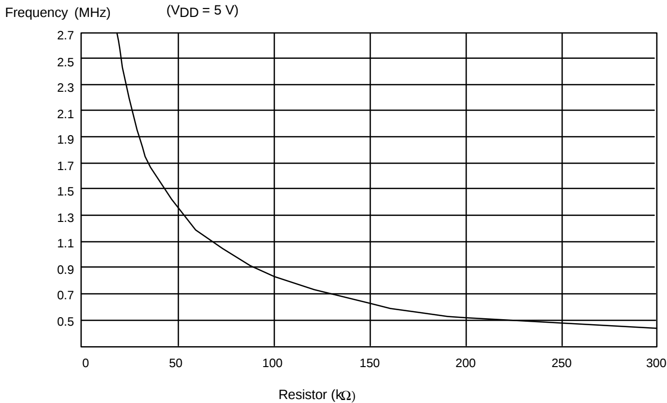
Figure 68. Frequency (fx) VS. Resistor
