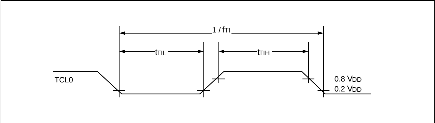
Figure 54. TCL Timing
