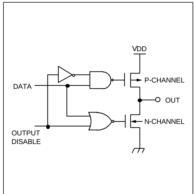
Figure 6. Pin Circuit Type 4
