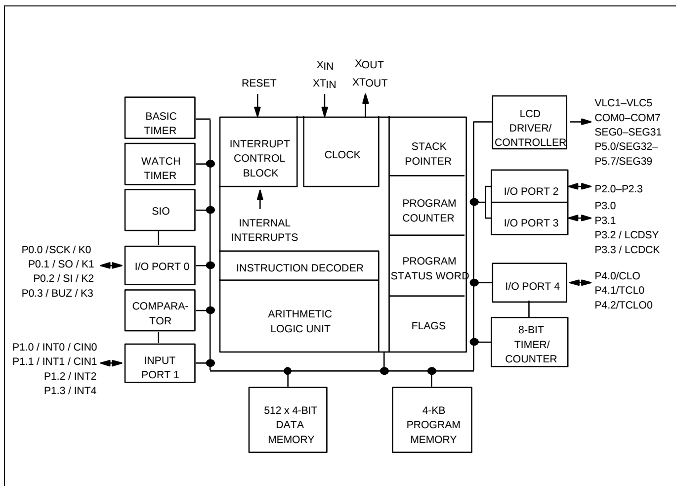
Figure 1. S3C7254 Simplified Block Diagram
