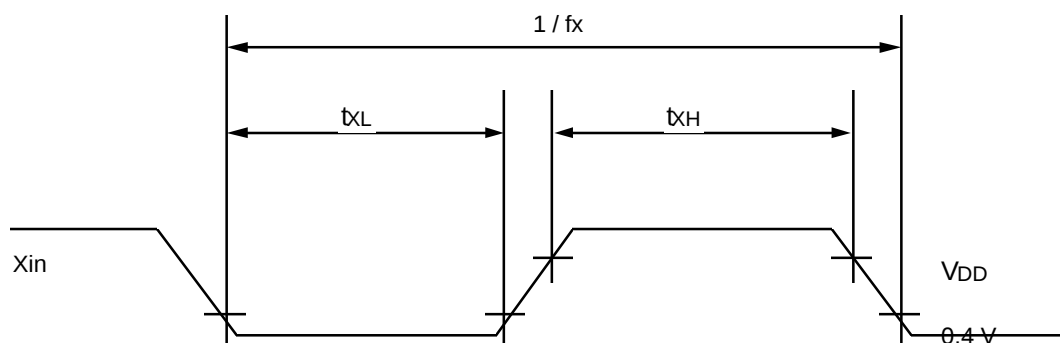
Figure 52. Clock Timing Measurement at X_{in}
