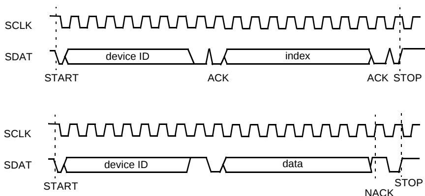
Figure 40. IIC Data Read
