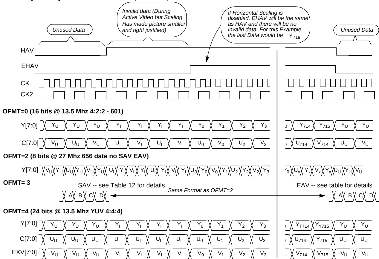
Figure 35. Horizontal Data Timing for Various Output Modes
