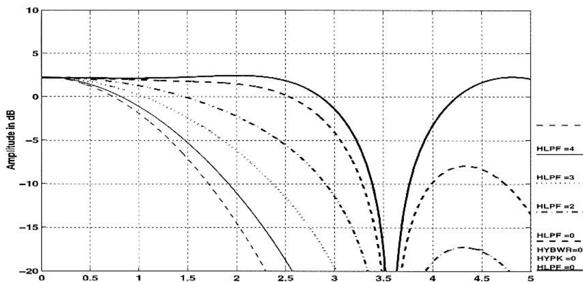
Figure 14. Medium to Low Frequency Luma Filter Characteristics (NTSC, CTAP=1)
