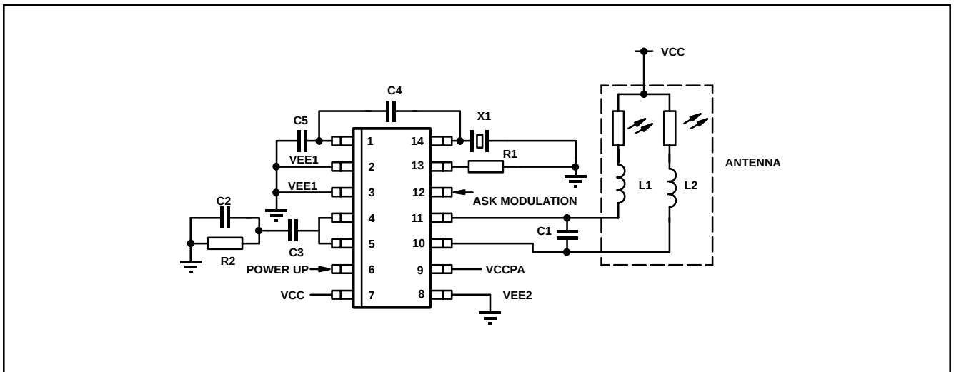
Figure 6 Application diagram
