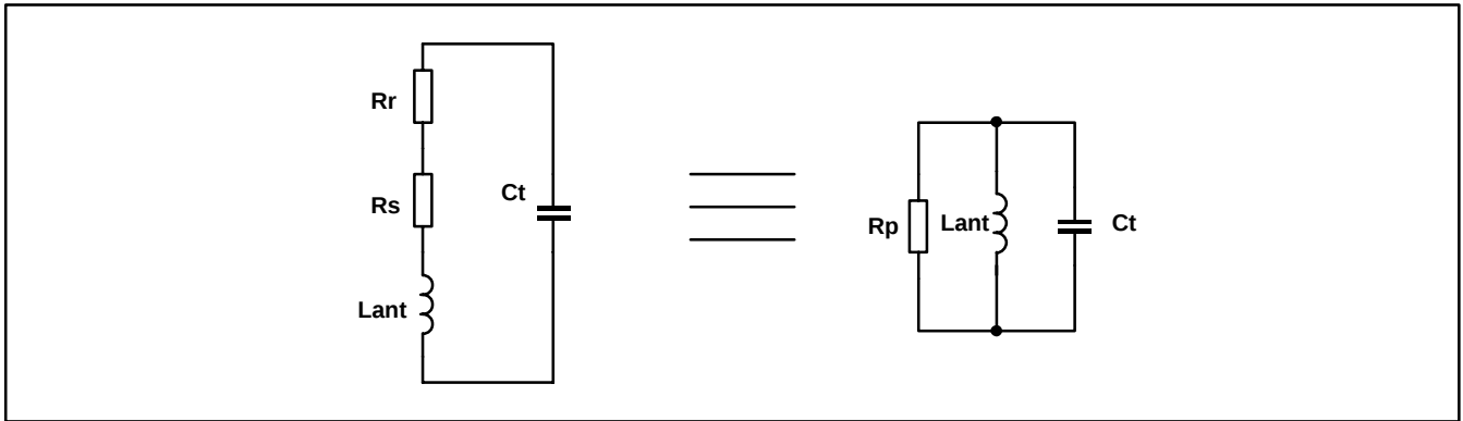
Figure 5 Loop antenna
