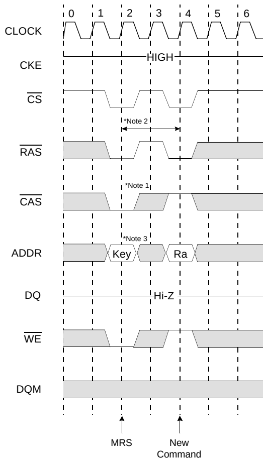
Mode Register Set Cycle
