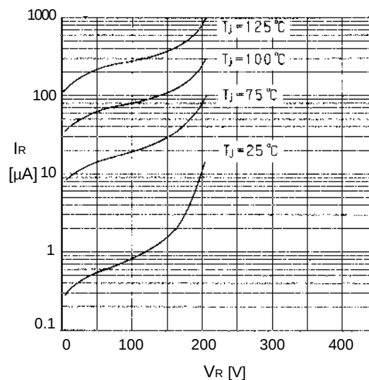
Reverse characteristics
