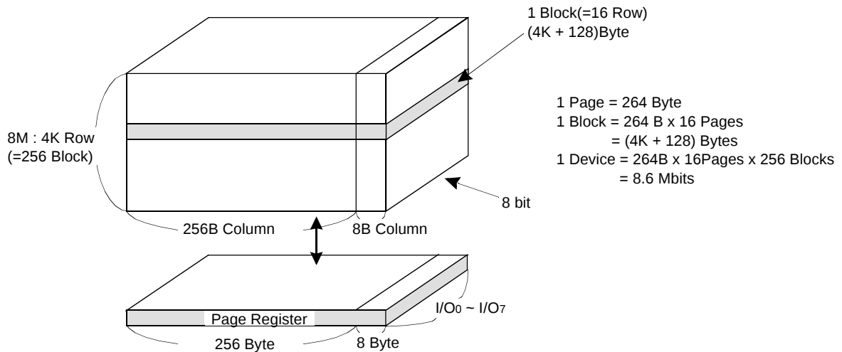
Figure 2. ARRAY ORGANIZATION
