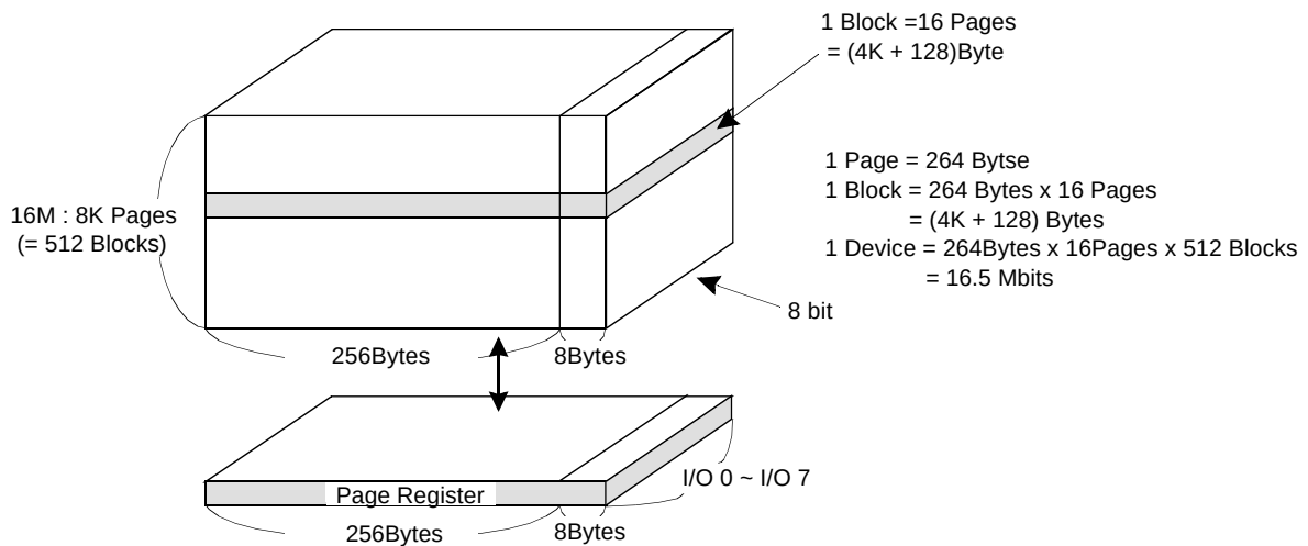
Figure 2. ARRAY ORGANIZATION
