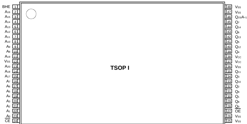
KM23V32005D(E)TY KM23S32005D(E)TY
