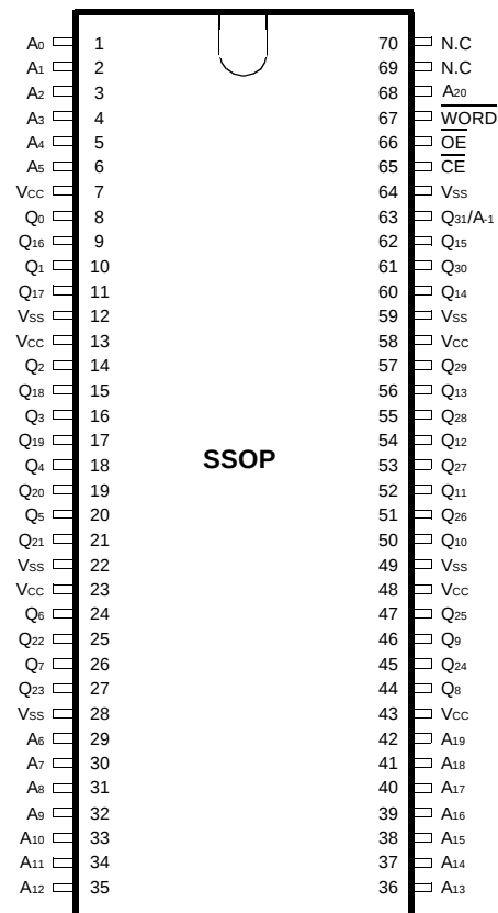
K3P7V(U)2000A-SC
