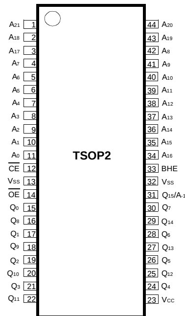
K3P7V(U)1000B-TC
