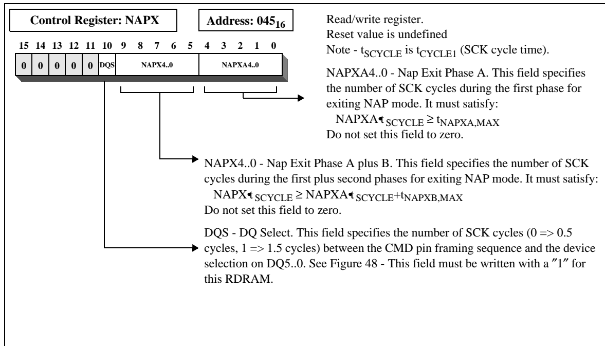
Figure 36: NAPX Register
