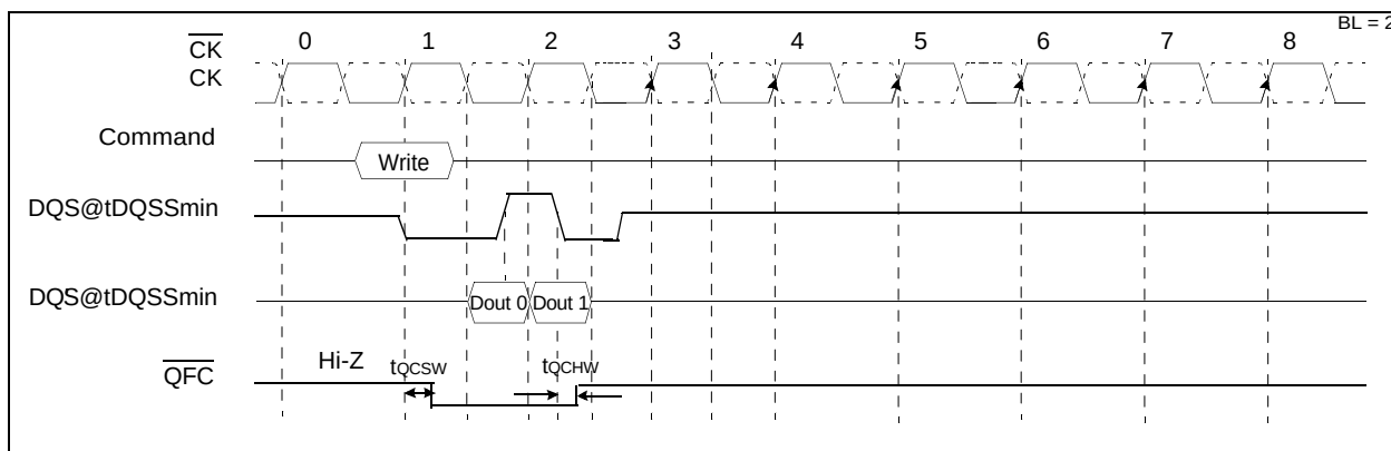
Figure 28. : \overline{QFC} timing on write operation with tDQSS_{min}
