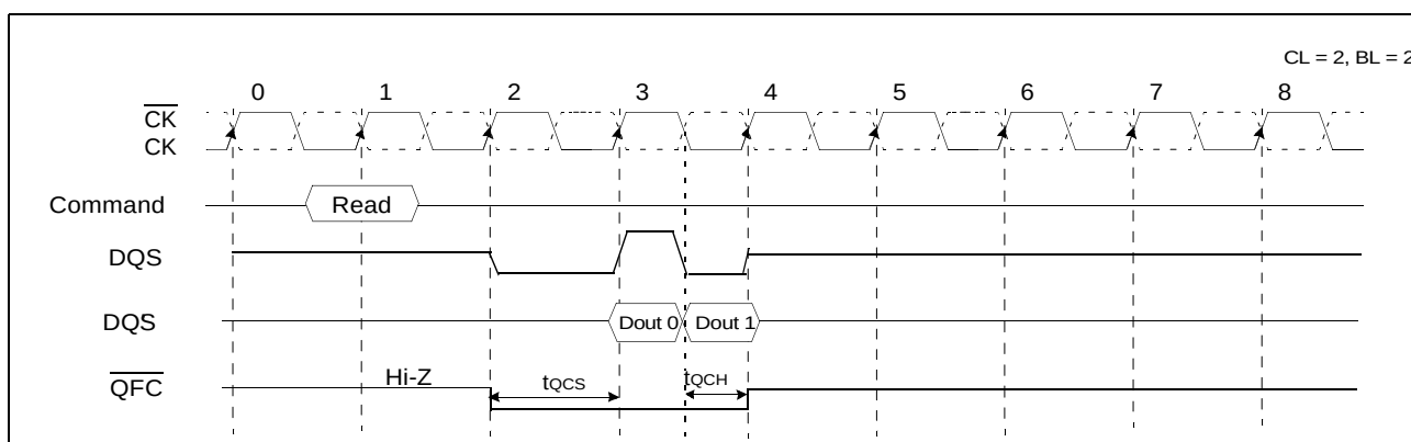
Figure 26. QFC timing on read operation
