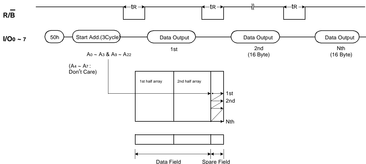
Figure 6. Sequential Row Read2 Operation (GND Input=Fixed Low) (K9F6408U0C-T or K9F6408U0C-V only)
