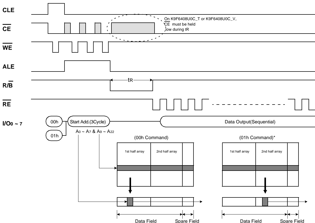
Figure 3. Read1 Operation
