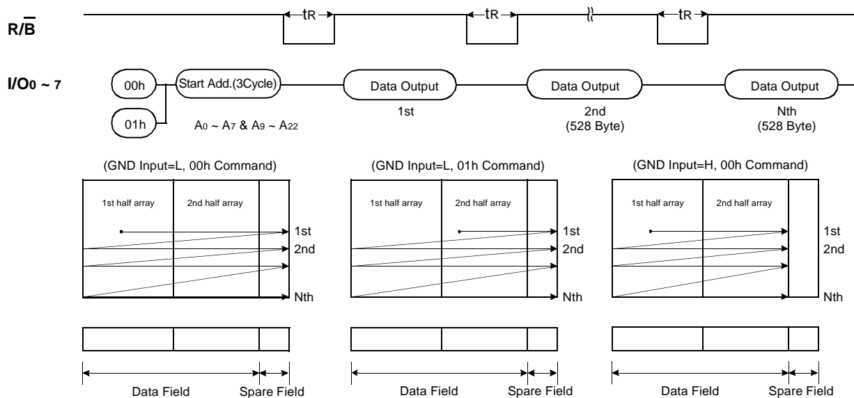
Figure 5. Sequential Row Read1 Operation (K9F6408U0C-T or K9F6408U0C-V only)
