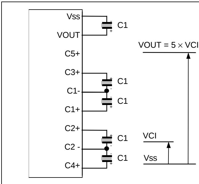
Figure 17. Five Times Boosting Circuit
