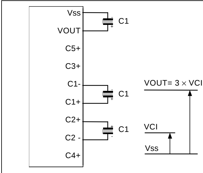
Figure 15. Three Times Boosting Circuit
