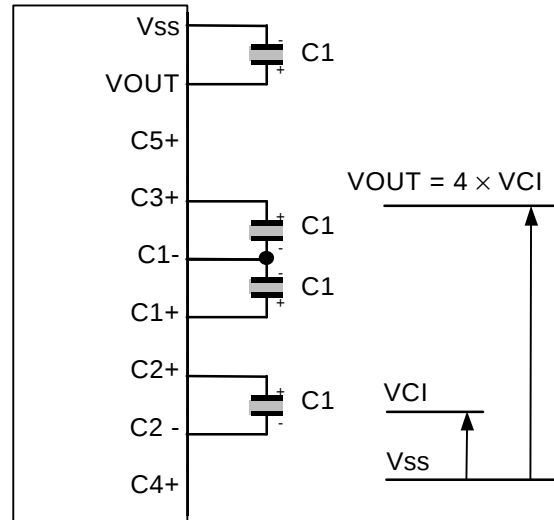
Figure 16. Four Times Boosting Circuit
