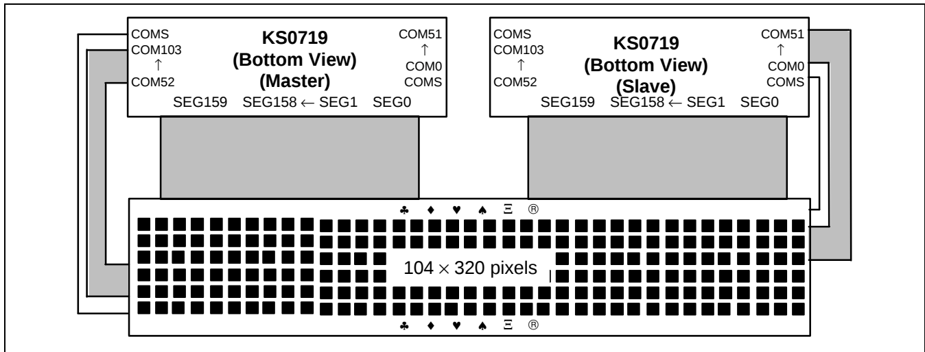
Figure 50. SHL = 0, ADC = 1
