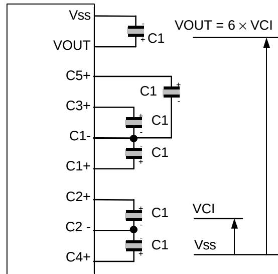
Figure 18. Six Times Boosting Circuit
