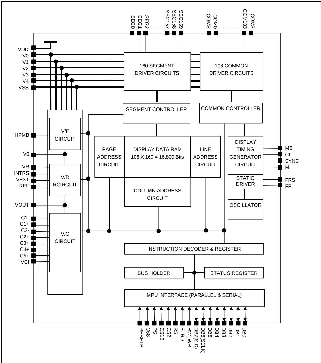
Figure 1. Block Diagram
