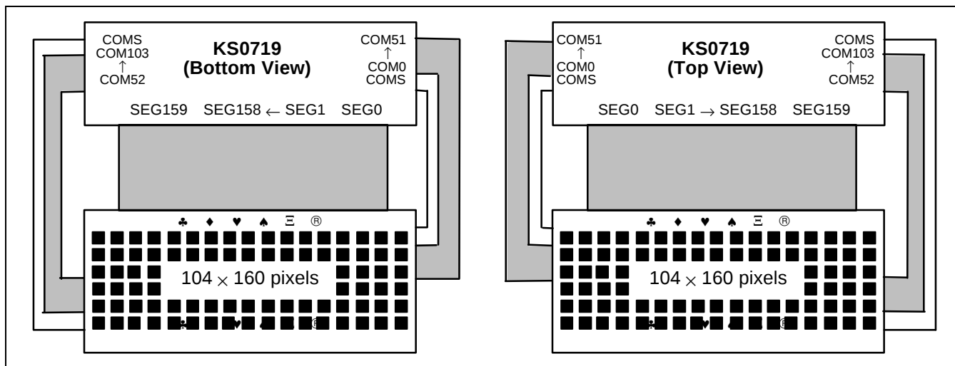
Figure 46. SHL = 0, ADC = 0
