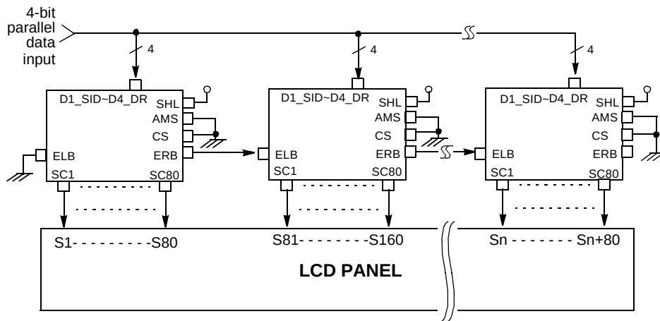
b) Upper View (SHL = H, AMS = L)
