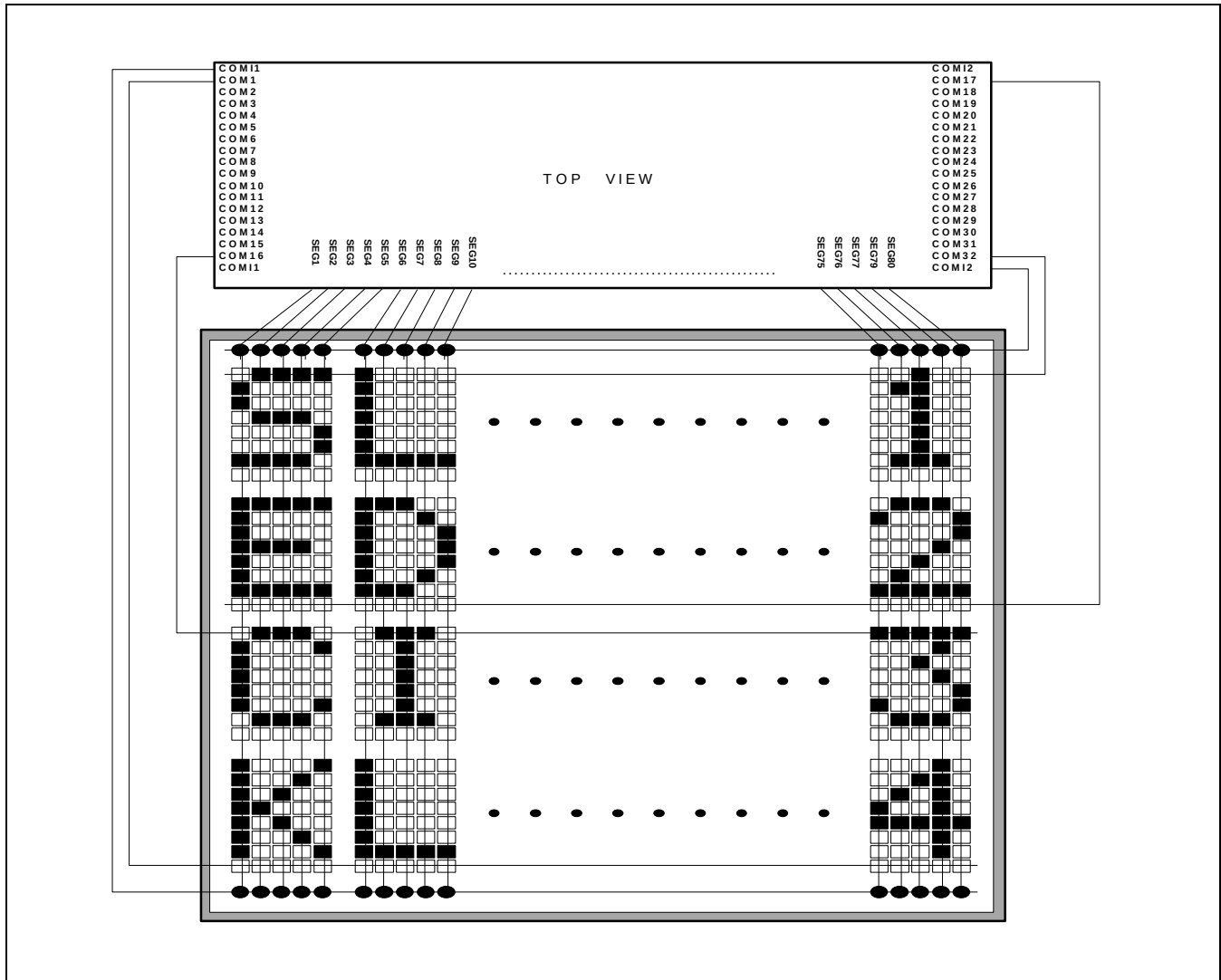
Figure 26. Chip Top &amp; Upper View (CS bit = "0", DIRS = "1")
