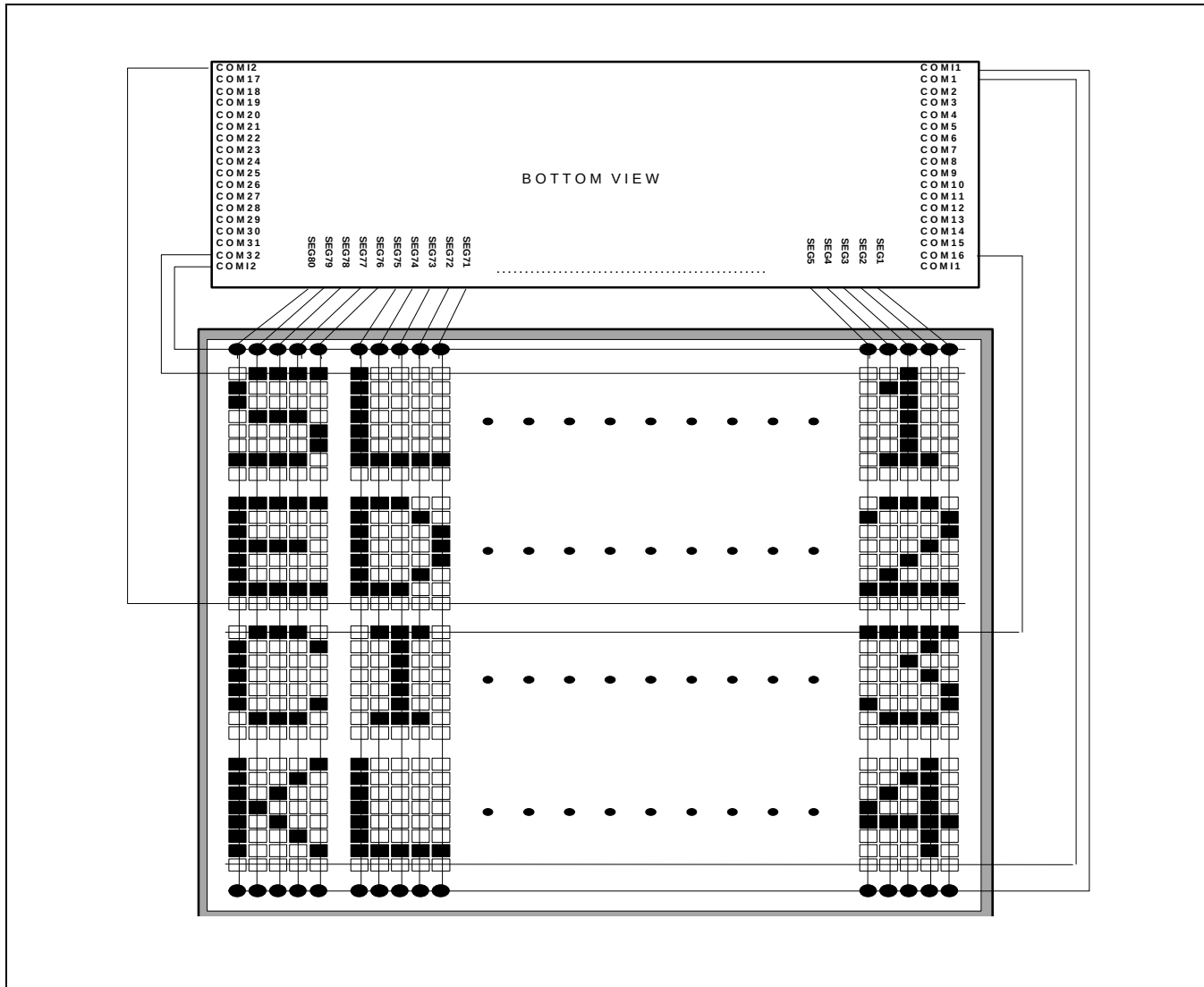
Figure 24. Chip Bottom &amp; Upper View (CS bit = "1", DIRS = "1")
