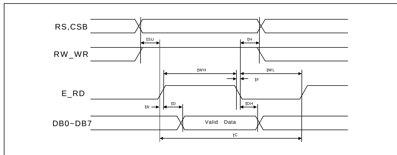
Figure 28. Read Timing Diagram (68-series)
