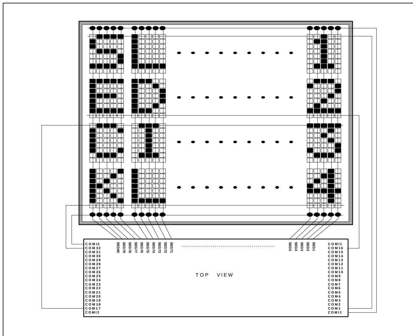
Figure 25. Chip Top &amp; Lower View (CS bit = "0", DIRS = "1")
