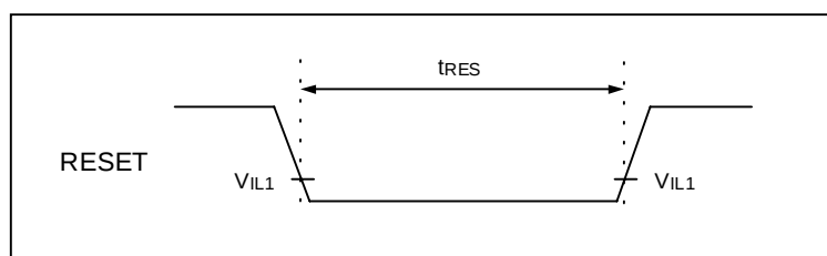
Fig-25. Reset TimingDiagram
