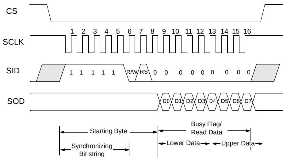
Fig-19. Timing Diagram of Serial Data Transfer
