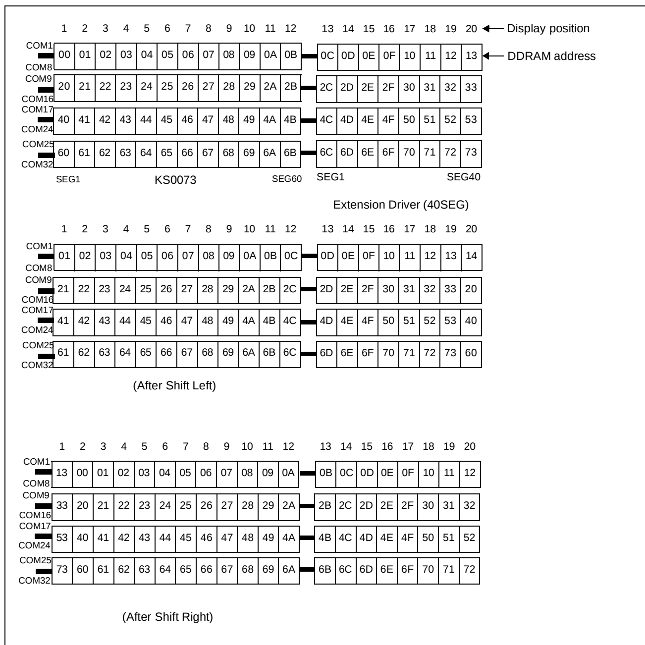
Fig-7. 4-line × 20 char. display with 40 SEG. extension driver (5-dot font width)
