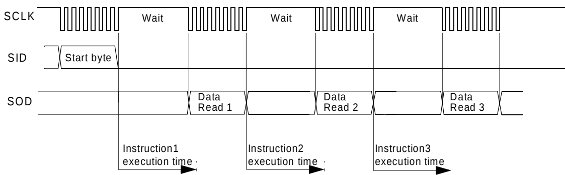
Fig-20. Timing Diagram of Continuous Data Transfer
