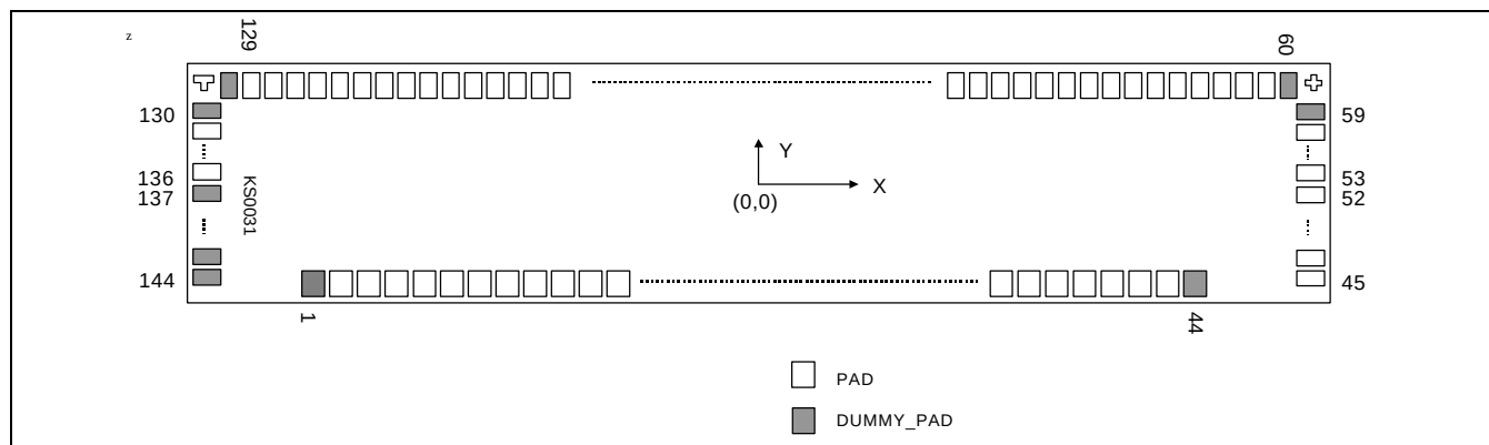
Figure 2. KS0031 Chip Configuration
