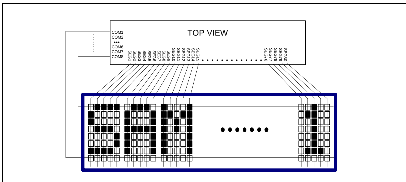
Figure 16. Chip Top &amp; Upper View Interfacing with LCD Panel
