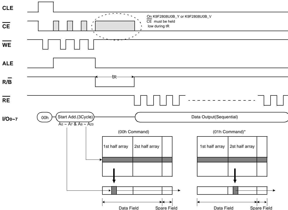
Figure 7. Read1 Operation
