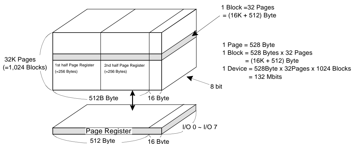
Figure 2. ARRAY ORGANIZATION
