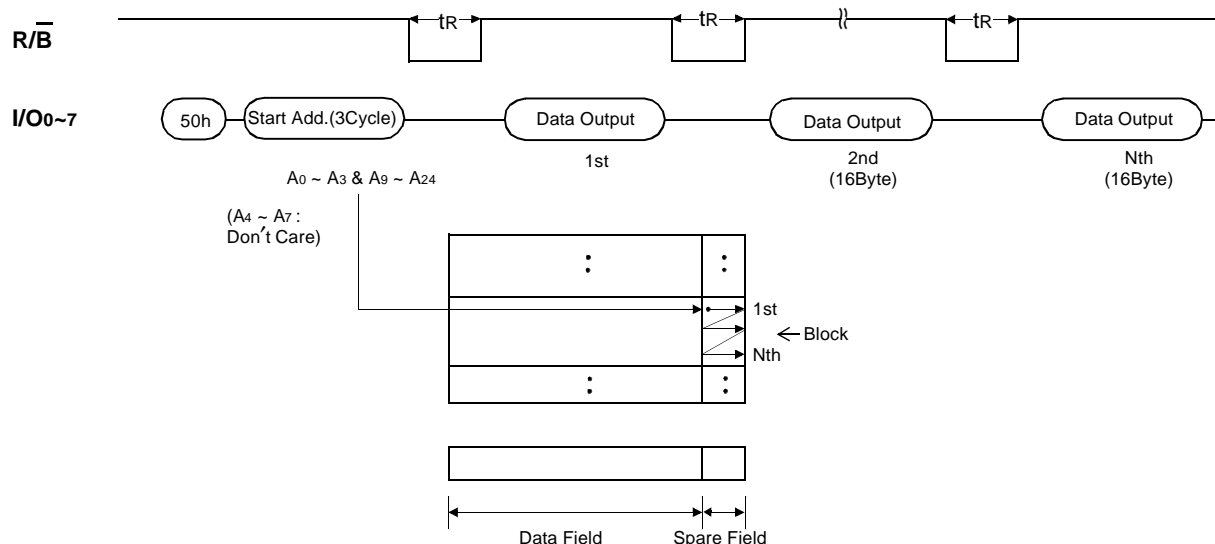
Figure 8-1. Sequential Row Read2 Operation (GND Input=Fixed Low) (only for K9F2808U0B-Y or K9F2808U0B-V)
