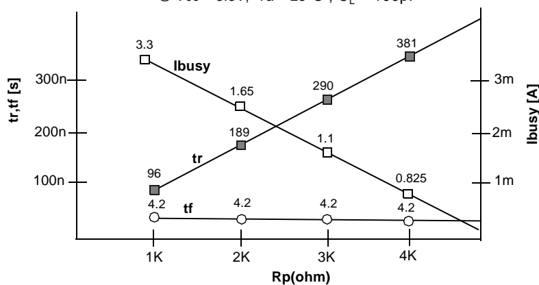
Figure 13. R_p vs t_r, t_f & R_p vs i_{busy}
