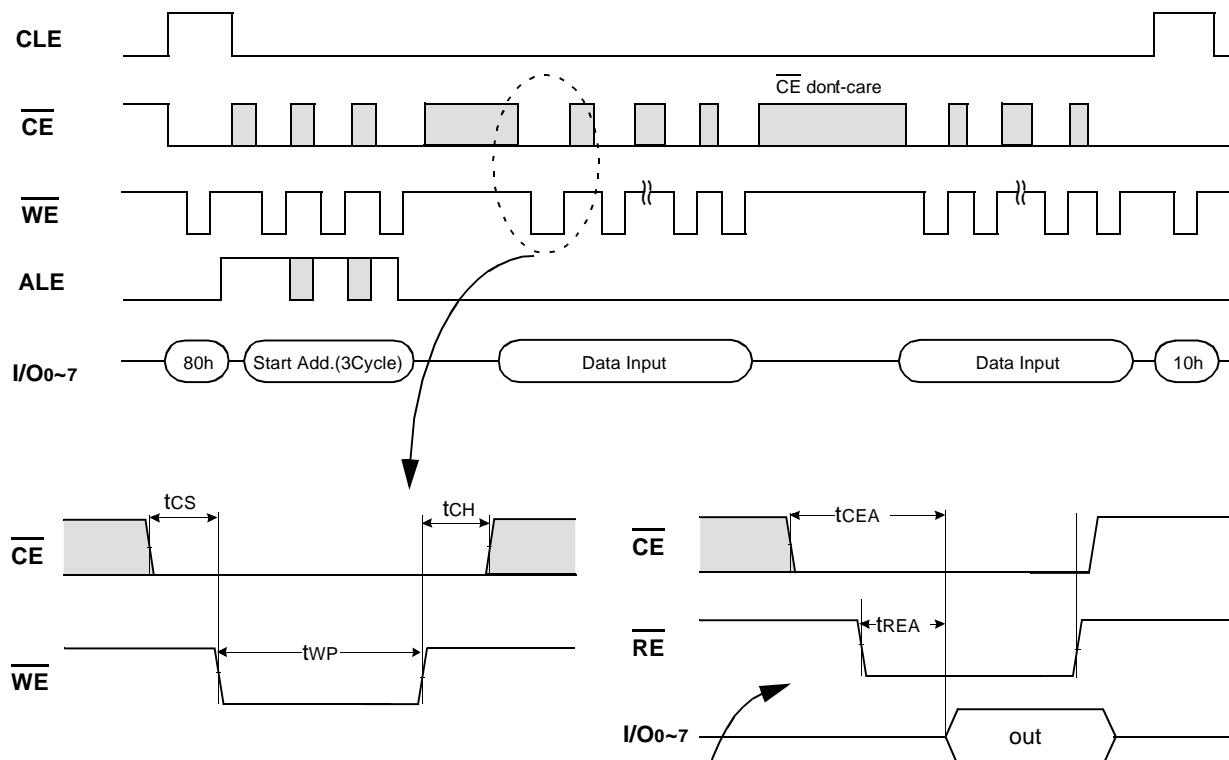
Figure 5. Program Operation with \overline{\text{CE}} dont-care.
