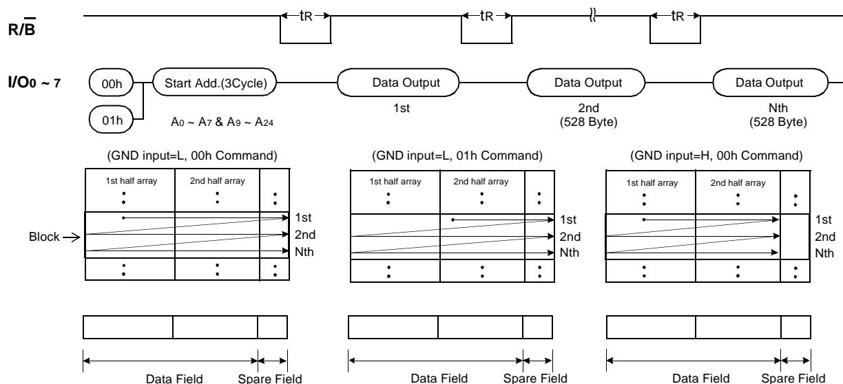
Figure 7-1. Sequential Row Read1 Operation ( only for K9F2808U0B-Y or K9F2808U0B-V )
