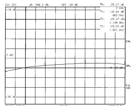
KEK-706H (COUPLING)
