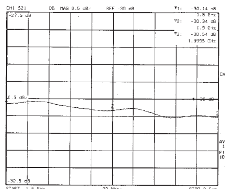
KEK-705H (COUPLING)
