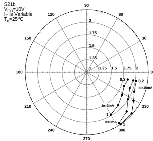
Figure 12. S21
