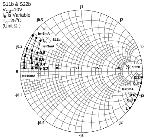
Figure 11. S11 & S22
