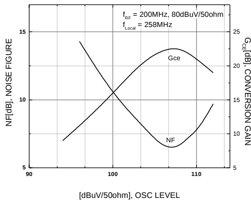
Figure 11. NF, G_{ce} - \text{OSC Level}
