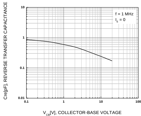
Figure 5. C_{re} - V_{CB}
