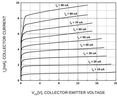
Figure 1. Static Charateristics
