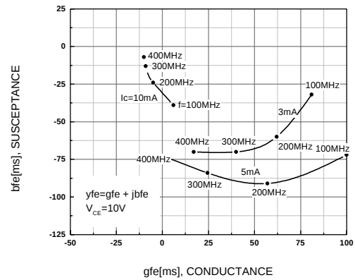
Figure 10. y_{fe} - f
