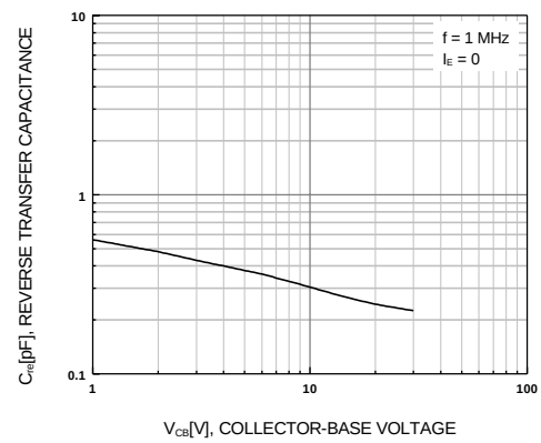
Figure 6. C_{re} - V_{CB}
