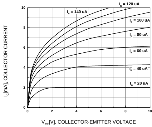
Figure 1. Static Characteristics
