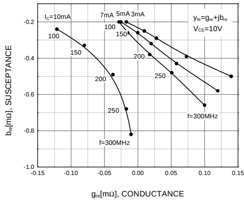
Figure 7. Reverse Transfer Admittance (yre) vs. Frequency
