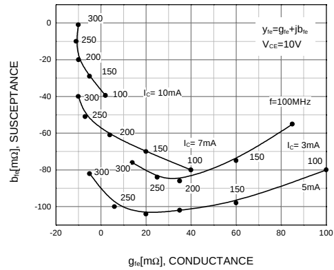
Figure 8. Forward Transfer Admittance ( y_{fe} ) vs. Frequency
