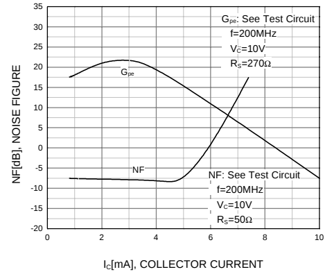
Figure 10. Power Gain and Noise Figure vs. Collector Current
