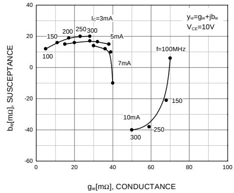
Figure 6. Input Admittance ( y_{ie} ) vs. Frequency
