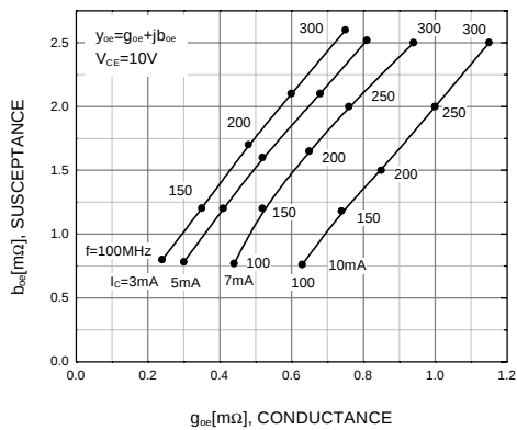
Figure 9. Output Admittance (yoe) vs. Frequency
