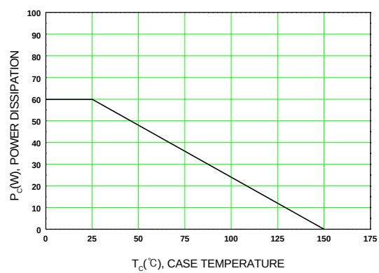
Figure 6. Power Derating
