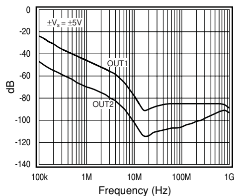
Figure 9: +V_b PSRR
