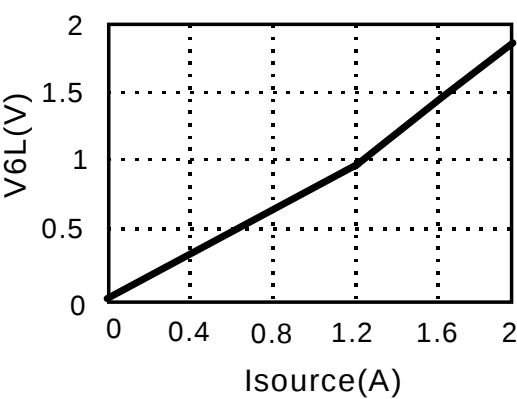
Figure 4. Isource-V6L
