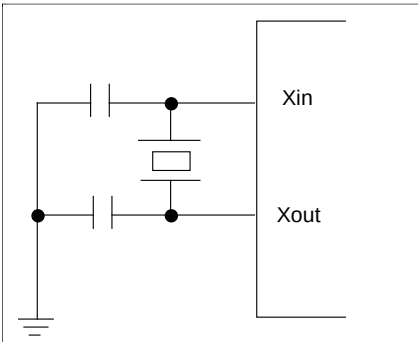
Figure 17. Crystal/Ceramic Oscillator
