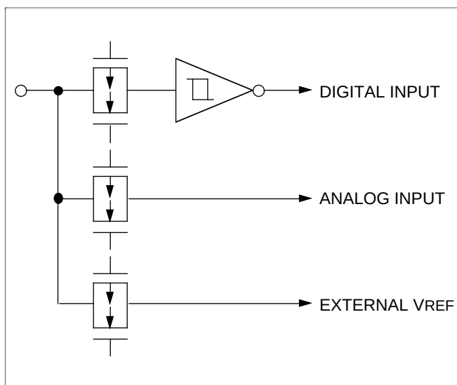
Figure 10. Pin Circuit Type 8
