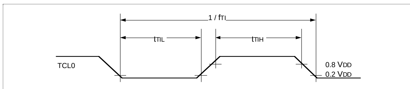
Figure 41. TCL0 Timing
