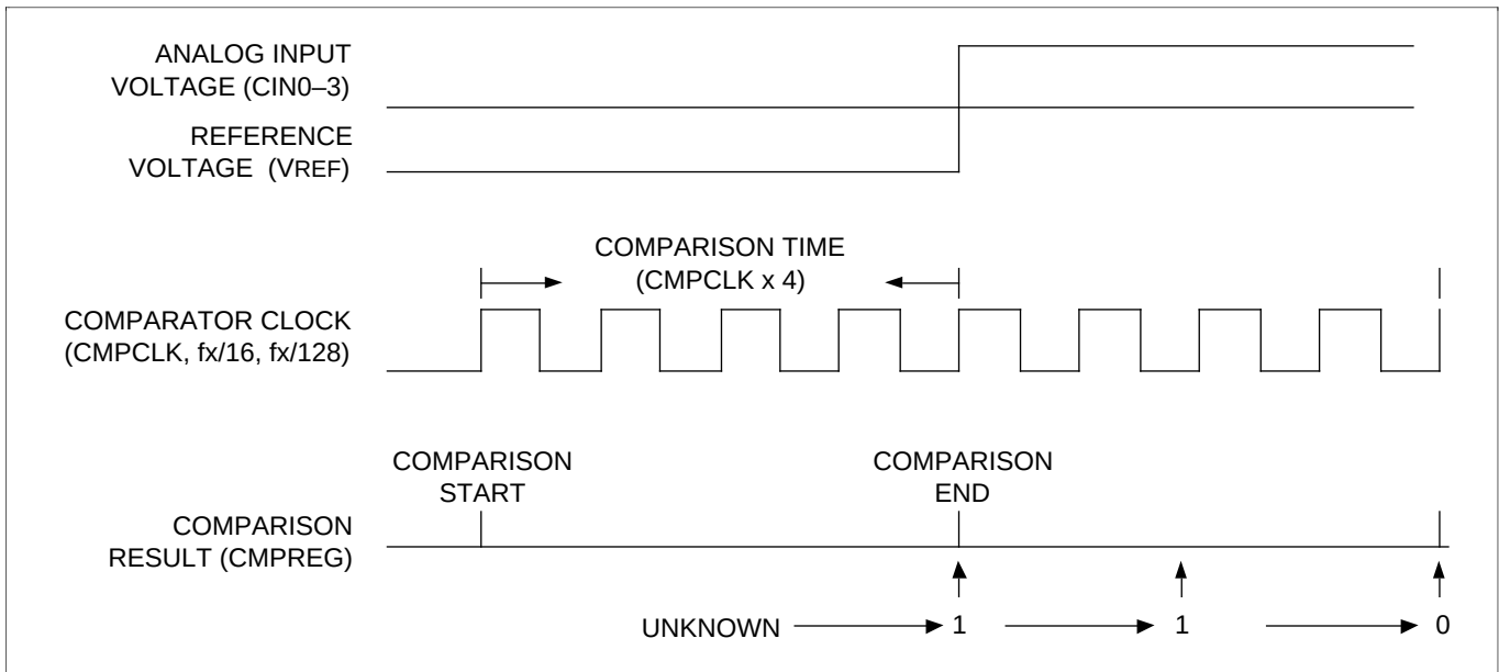
Figure 32. Conversion Characteristics
