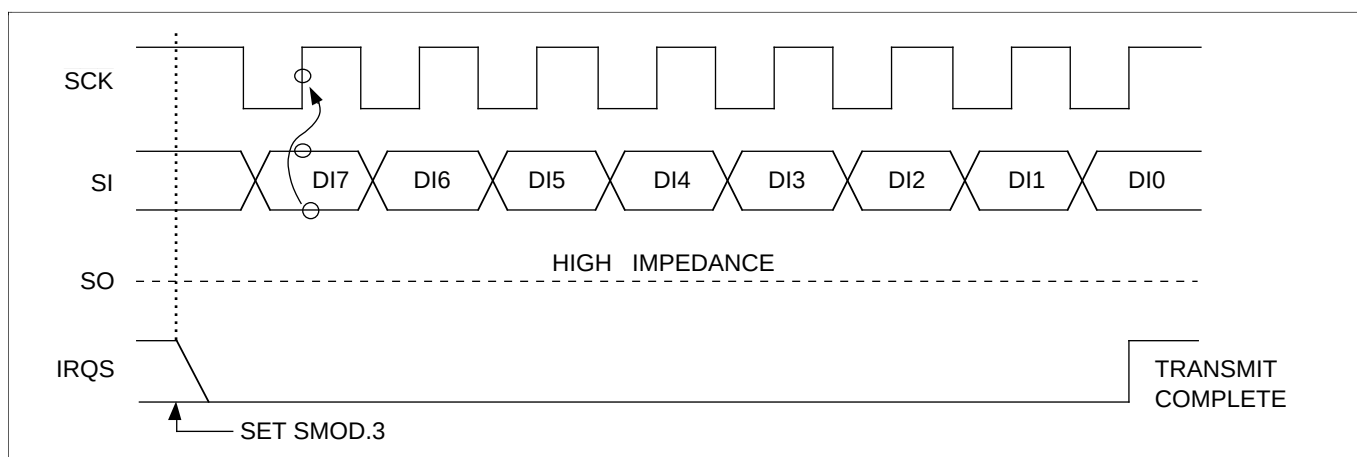
Figure 35. SIO Timing in Receive-Only Mode
