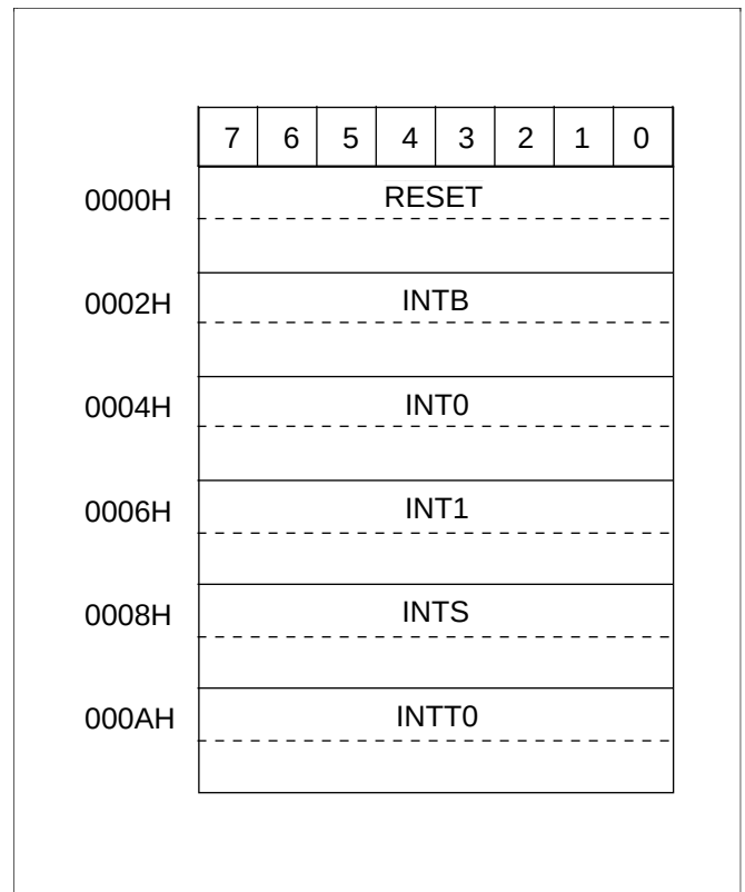
Figure 13. Vector Address Map
