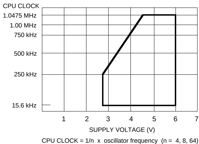
Figure 36. Standard Operating Voltage Range
