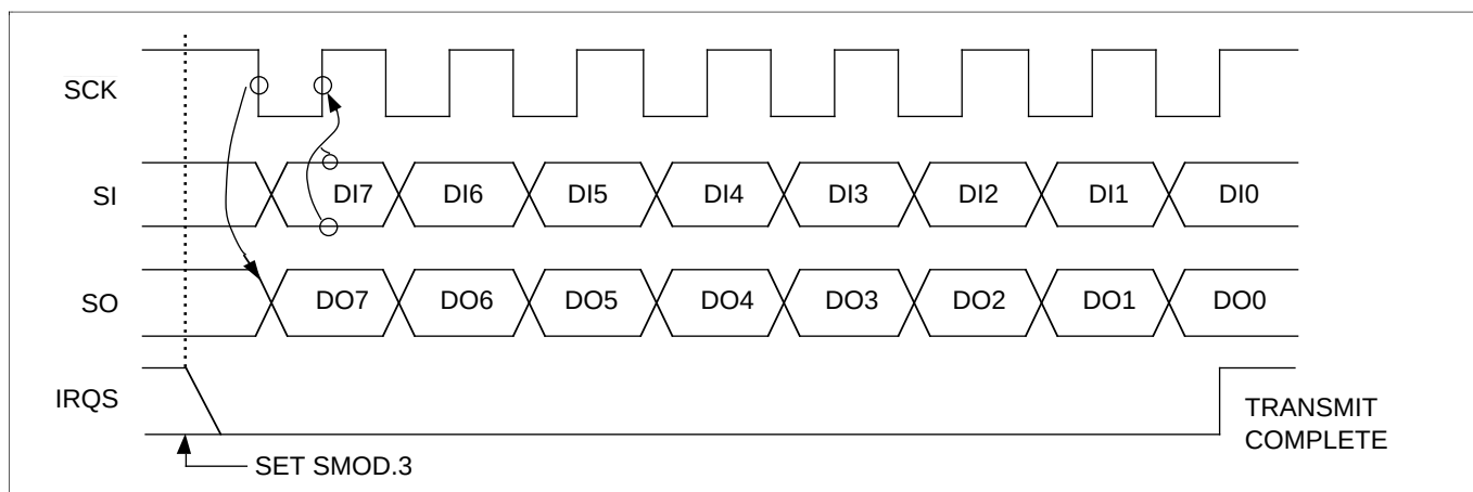
Figure 34. SIO Timing in Transmit/Receive Mode
