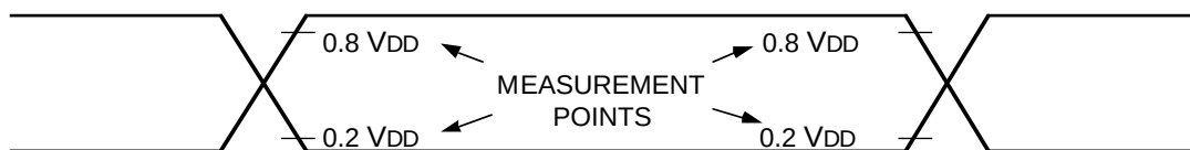
Figure 37. A.C. Timing Measurement Points (Except for X in )
