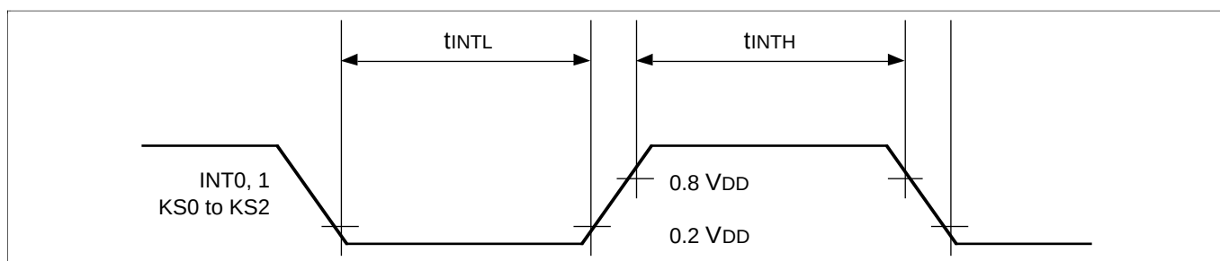
Figure 43. Input Timing for External Interrupts
