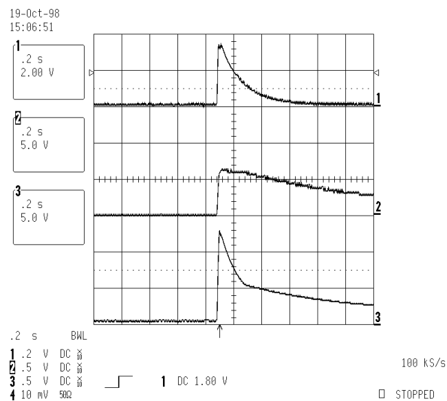
Figure 24. No Load Protection
