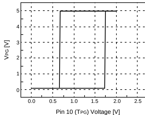
Figure 18. Hysteresis Voltage 2
