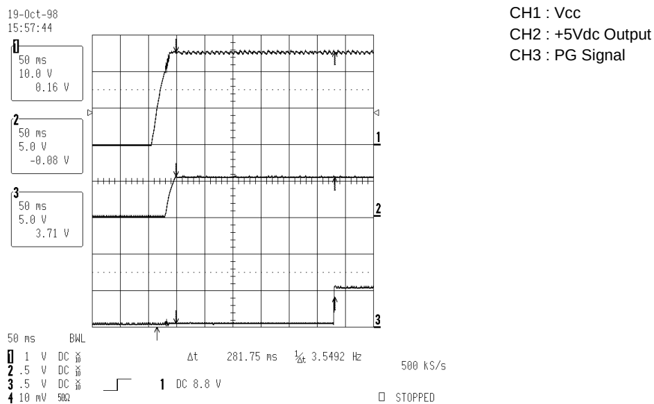
Figure 26. Vcc, +5Vdc Output vs. PG Signal (Low)
