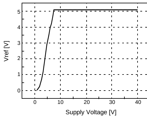
Figure 20. Reference Voltage
