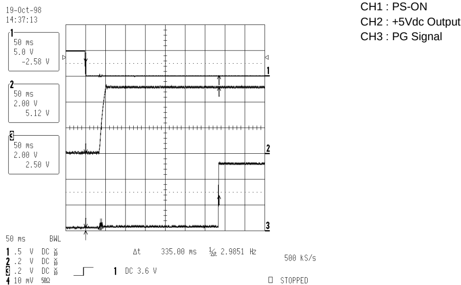
Figure 22. PG Signal Delay Time
