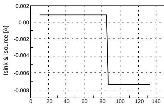
Figure 19. Error Amp Sink Current
