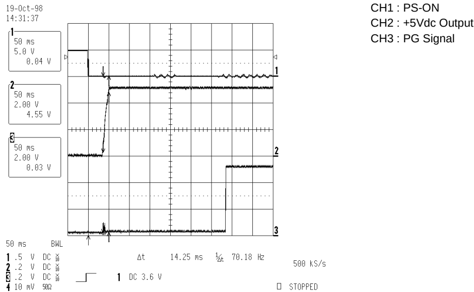
Figure 21. Rising Time of +5Vdc Output Voltage
