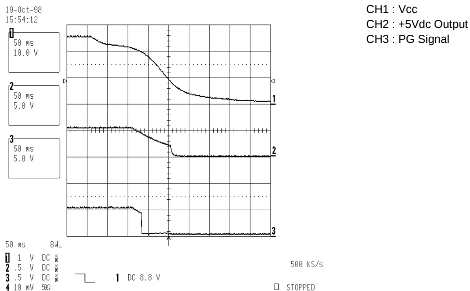
Figure 25. Vcc, +5Vdc Output vs. PG Signal (High)
