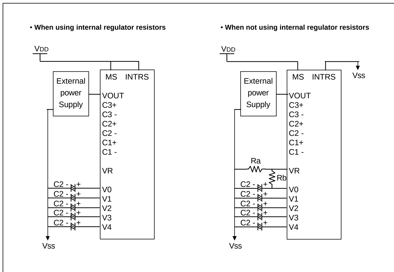
Figure 13. When Using Some LCD Power Circuits (V/C: Off, V/R: On, V/F: On)
