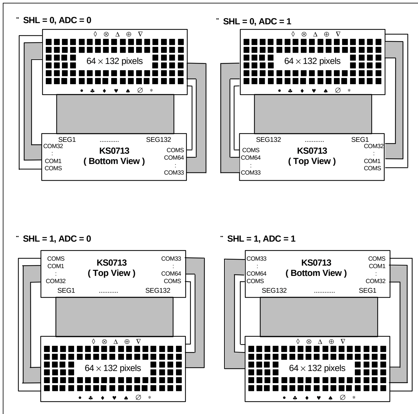
Figure 29. Single-Chip Structure (1/65 Duty Configurations)
