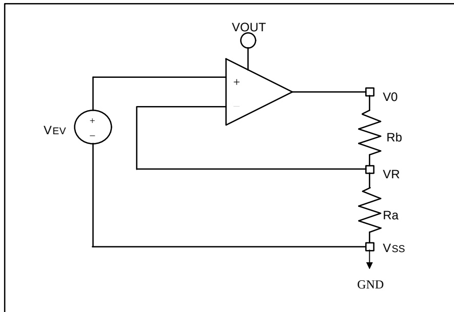
Figure 10. Internal Voltage Regulator Circuit
