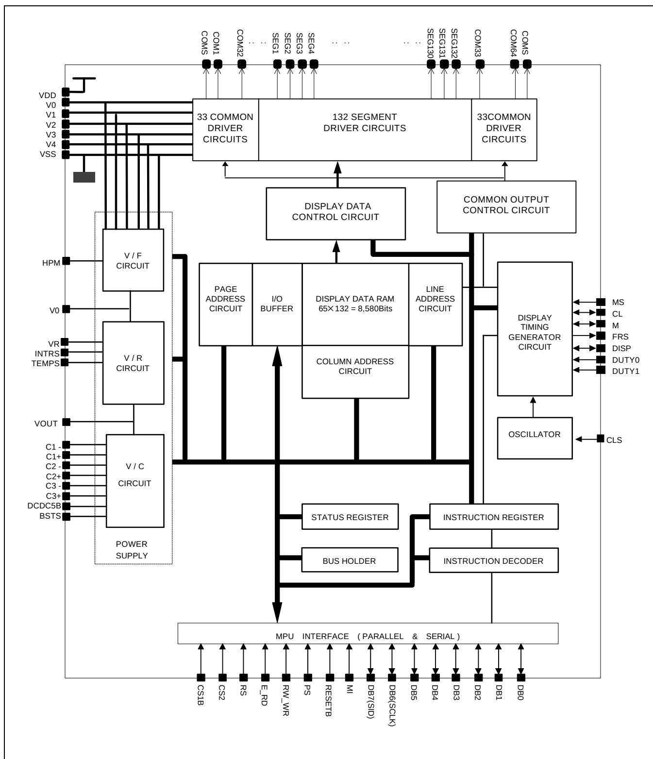
Figure 1. Block Diagram
