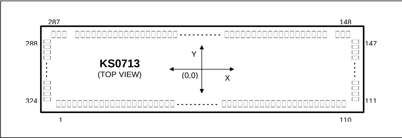
Figure 2. Pad Configuration
