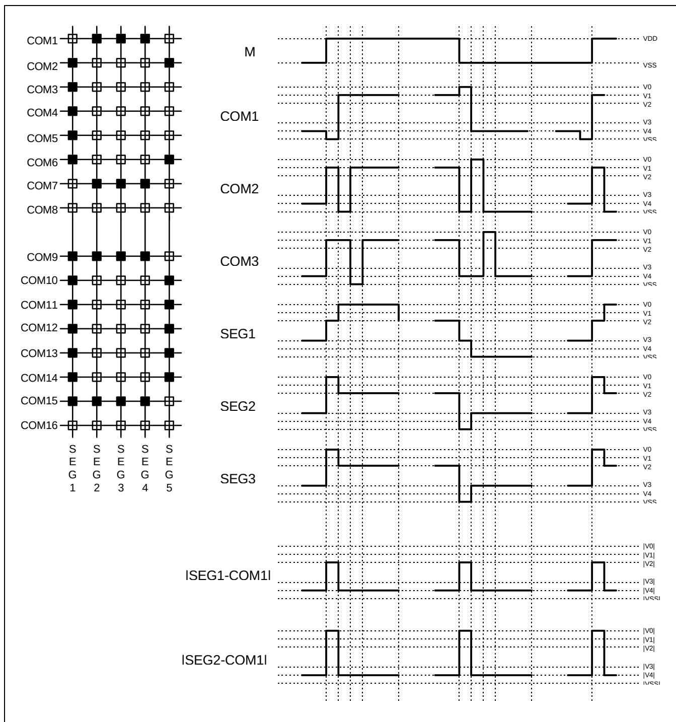
Figure 8. Segment and Common Timing
