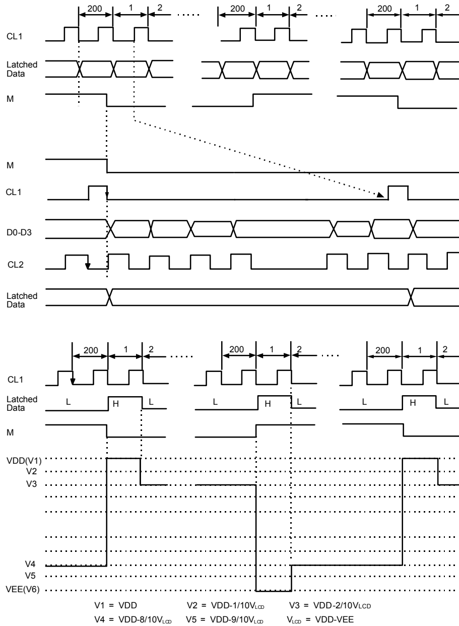
Timing Chart - 1/200 Duty, 1/15 Bias
