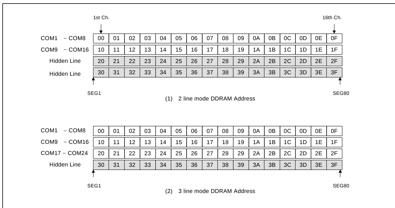
Figure 8. DDRAM Address
