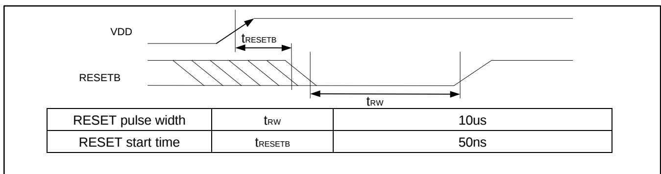
Figure 17. RESET Timing
