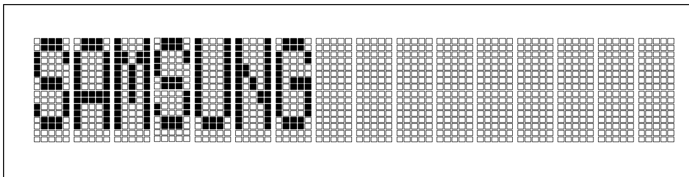
Figure 14. COM1 ~ 16 is a double height line ( DH2,DH1 = 01)
