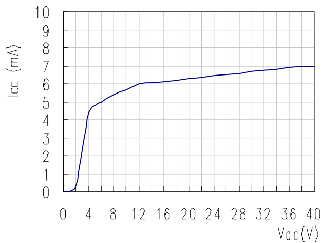
2. V_{CC} vs I_{CC}
