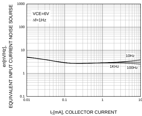
Figure 9. Equivalent Input Current Noise Source
