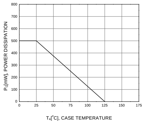
Figure 11. Power Derating
