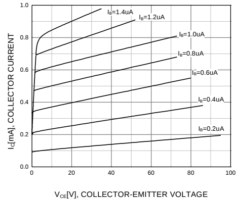
Figure 2. Static Characteristic
