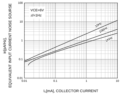
Figure 8. Equivalent Input Current Noise Source
