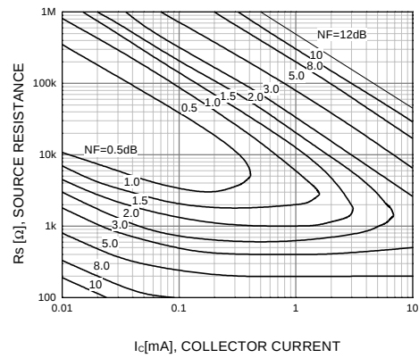
Figure 10. Noise Figure MHP
