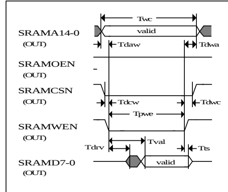
Figure 4.2.1 SRAM Write AC Timing
