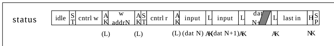
Figure 6.5.1 SEP Sequential Read Timings
