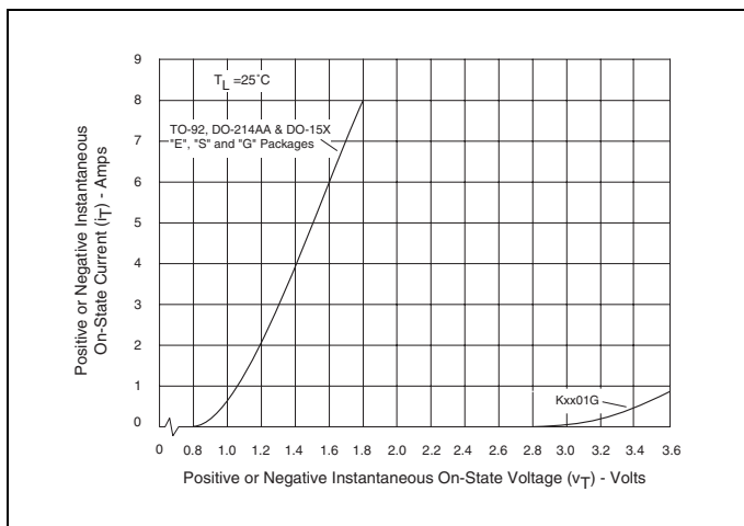
Figure 9.7 On-State Current vs On-State Voltage (Typical)
