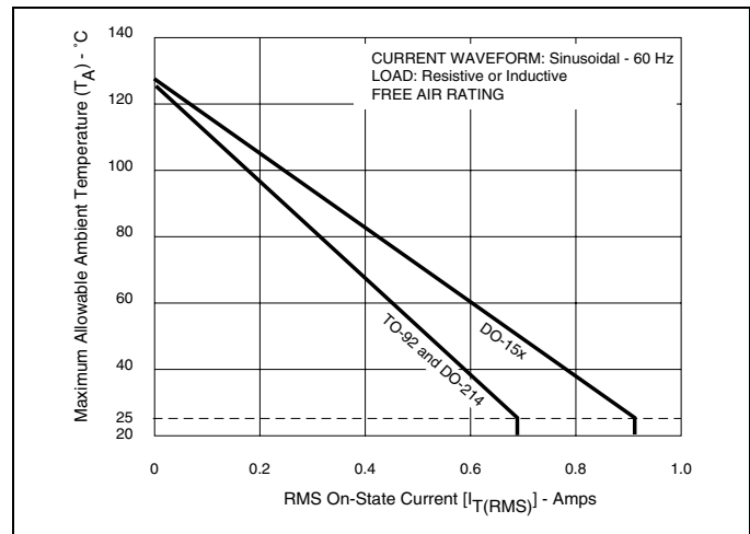
Figure 9.4 Maximum Allowable Ambient Temperature vs On-State Current
