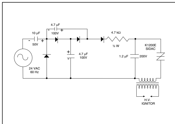
Figure 9.10 Ignitor Circuit (Low Voltage Input)
