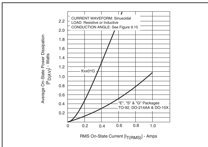
Figure 9.8 Power Dissipation (Typical) vs On-State Current
