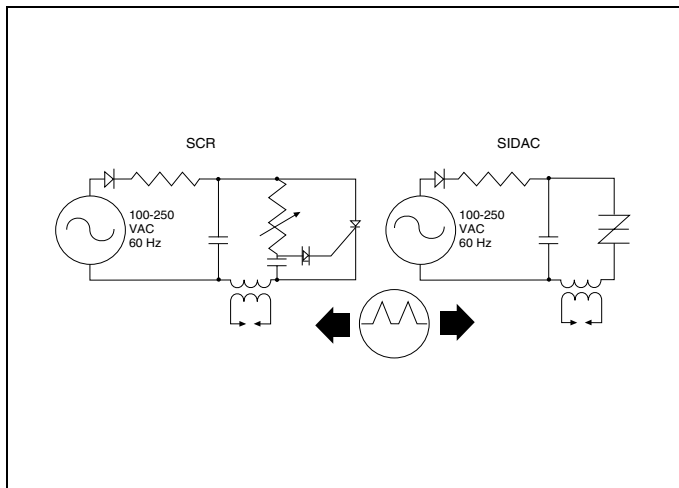
Figure 9.9 Comparison of Sidac vs SCR
