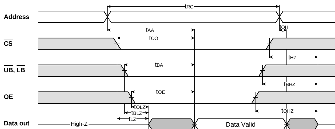
TIMING WAVEFORM OF READ CYCLE(2) ( \overline{\text{WE}}=\text{V}_{\text{IH}} )
