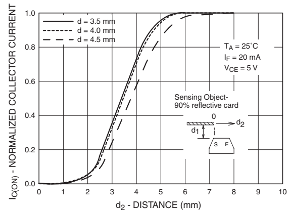
Normalized Collector Current vs. Distance d_2
