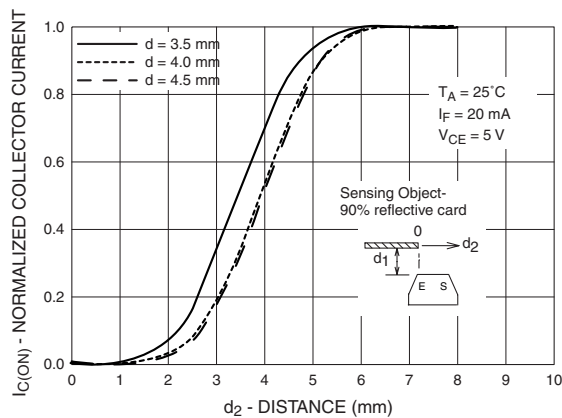
Normalized Collector Current vs. Distance d_2
