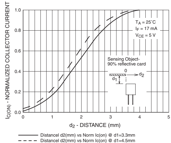
Normalized Collector Current vs. Distance d_2
