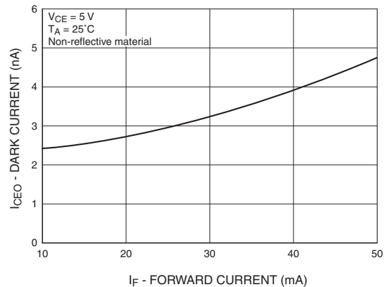
Collector Emitter Dark Current vs. Forward Current
