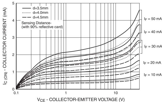
Collector Current vs. Collector to Emitter Voltage
