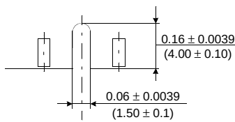
Detail Z
