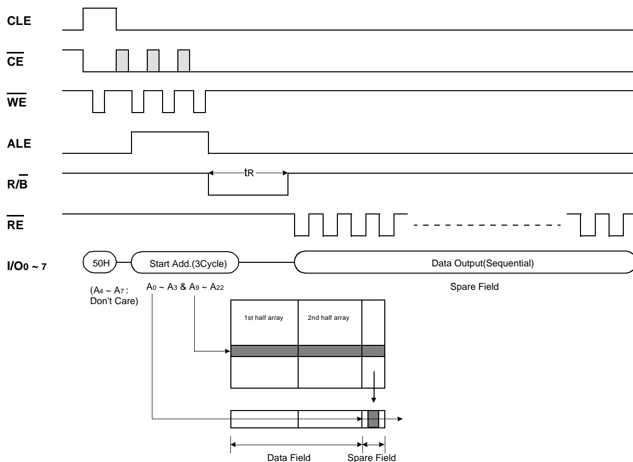
Figure 4. Read2 Operation
