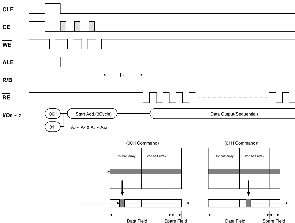
Figure 3. Read1 Operation
