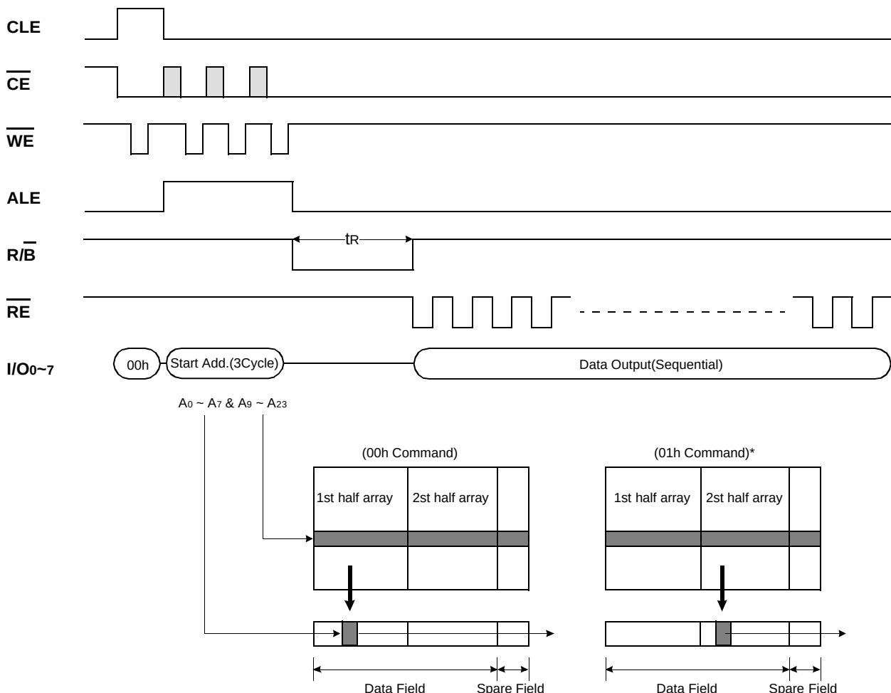
Figure 3. Read1 Operation
