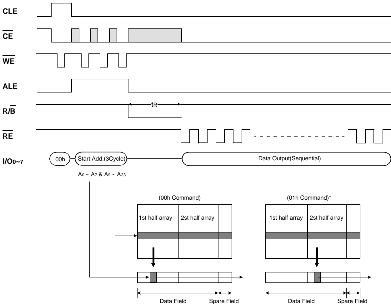
Figure 7. Read1 Operation
