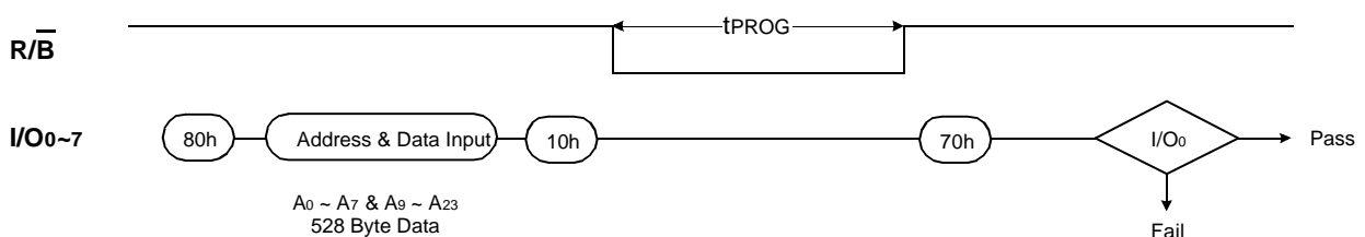
Figure 9. Program &amp; Read Status Operation
