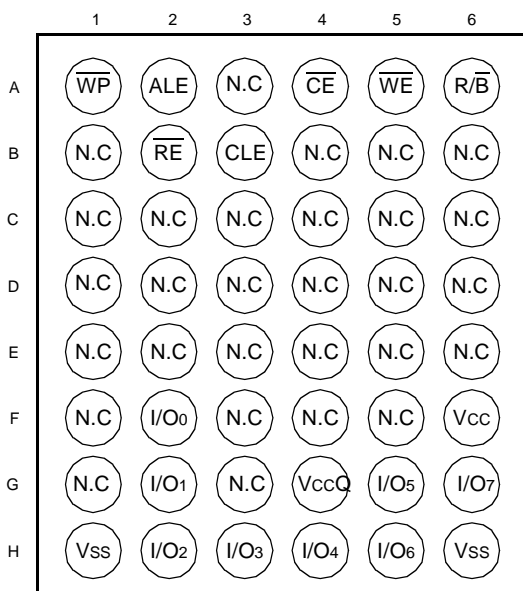
48 Ball TBGA , 0.8mm Pitch TOP View
