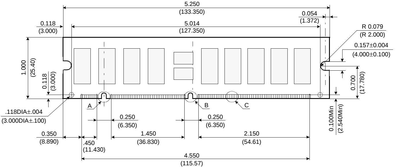
( Front view )
