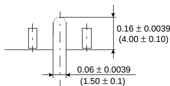
Detail Z
