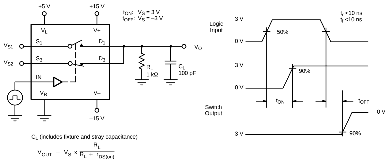
FIGURE 2. Switching Time
