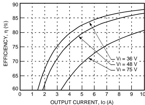
Figure 4. Typical JAHW050Y Converter Efficiency vs. Output Current at Room Temperature
