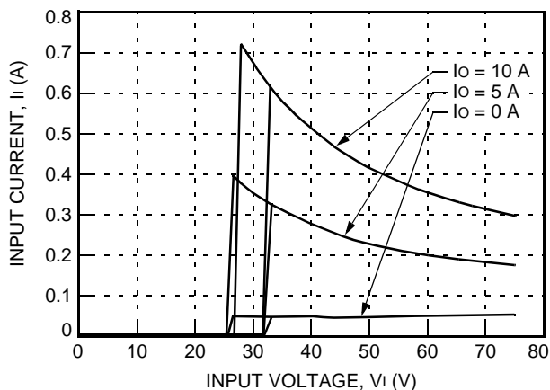
Figure 1. Typical JAHW050Y Input Characteristics at Room Temperature
