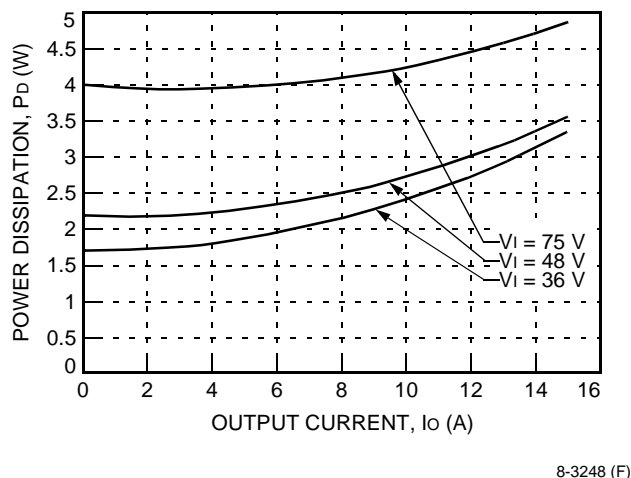
Figure 28. JAHW075Y Power Dissipation vs. Output Current at 25 °C
