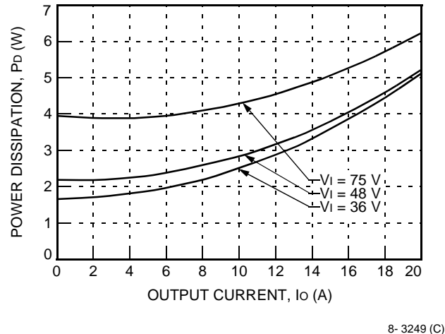
Figure 29. JAHW100Y Power Dissipation vs. Output Current at 25 °C
