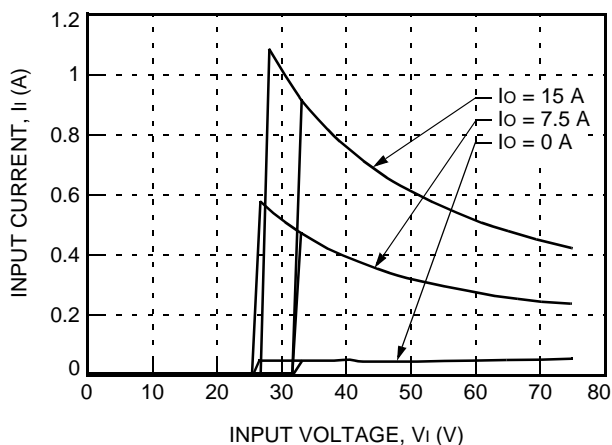
Figure 2. Typical JAHW075Y Input Characteristics at Room Temperature
