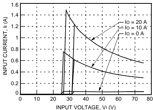
Figure 3. Typical JAHW100Y Input Characteristics at Room Temperature
