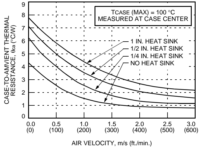
Figure 31. Case-to-Ambient Thermal Resistance Curves; Either Orientation
