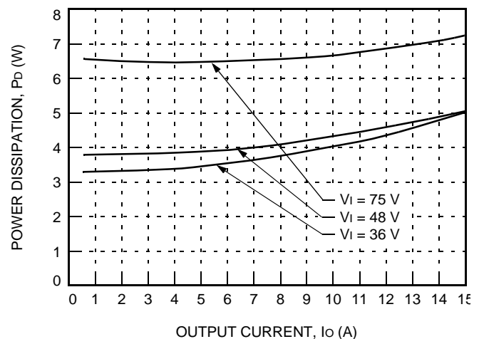
Figure 29. JAHW075G Power Dissipation vs. Output Current at 25 °C
