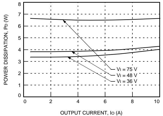
Figure 28. JAHW050G Power Dissipation vs. Output Current at 25 °C
