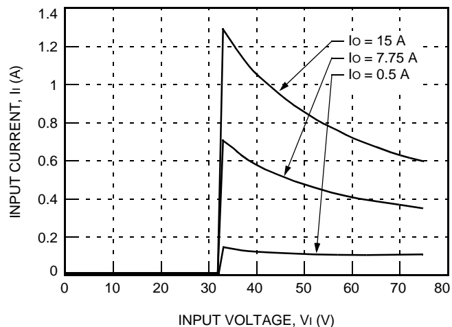
Figure 2. Typical JAHW075G Input Characteristics at Room Temperature
