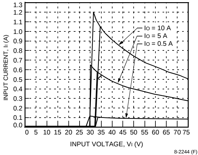
Figure 1. Typical JAHW050F-S Input Characteristics at Room Temperature
