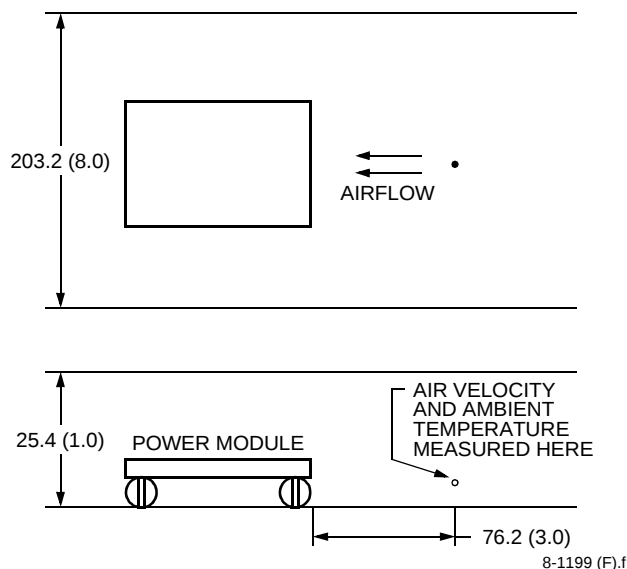
Figure 19. Thermal Test Setup
