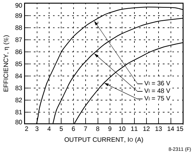
Figure 4. Typical JAHW075F-S Converter Efficiency vs. Output Current at Room Temperature
