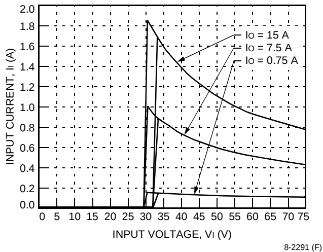
Figure 2. Typical JAHW075F-S Input Characteristics at Room Temperature
