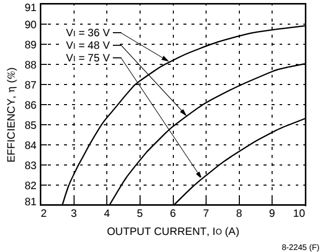
Figure 3. Typical JAHW050F-S Converter Efficiency vs. Output Current at Room Temperature
